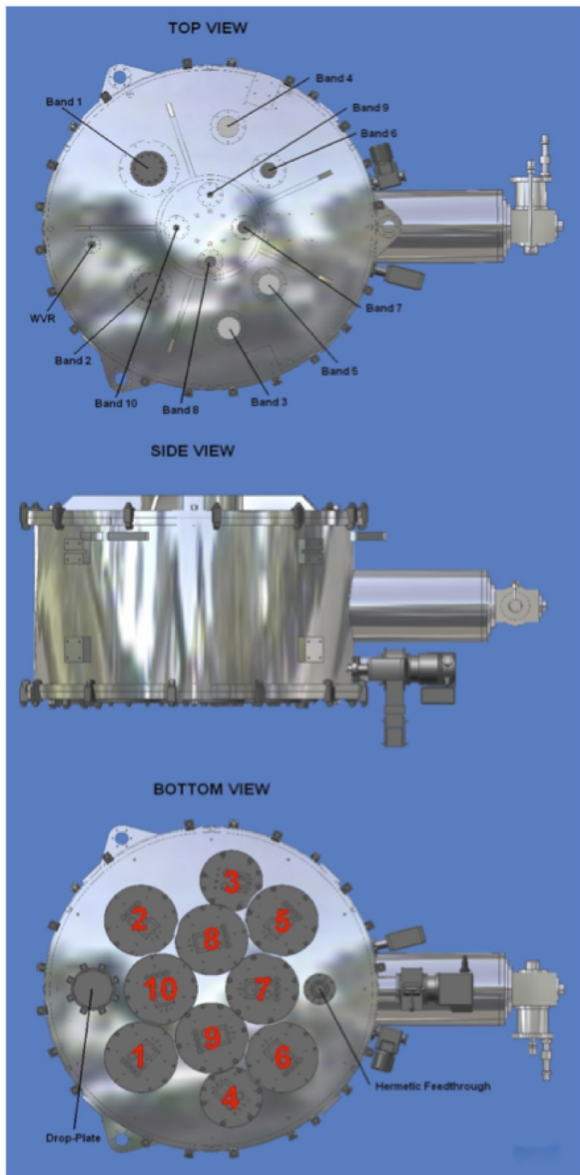
Figure A.6: Views of cryostat assembly, showing different windows (top) and the portholes for the WCs for each band (lower view).
